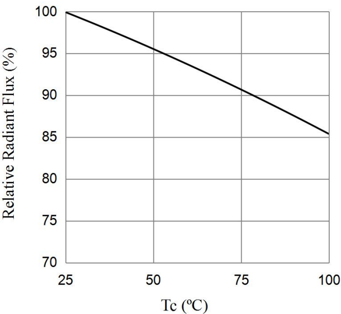
Case Temperature vs. Relative Radiant Flux ( I_f=1440\text{mA} )
